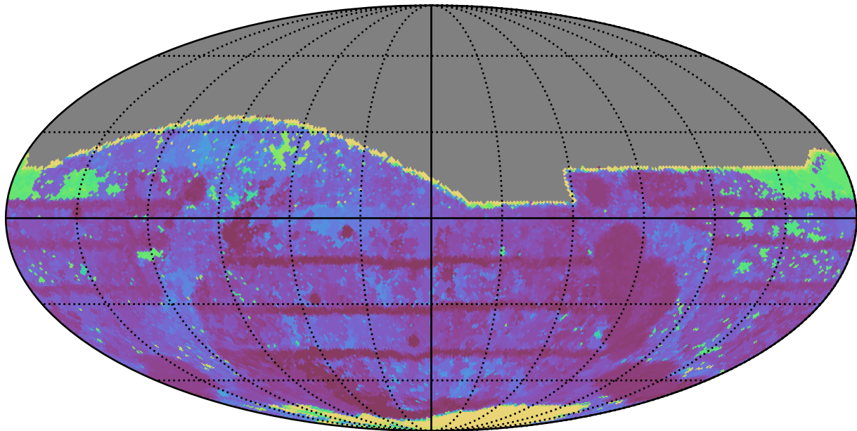
weather_cloudso30v3.4_10yrs All sky r band: Max Inter-Night Gap
