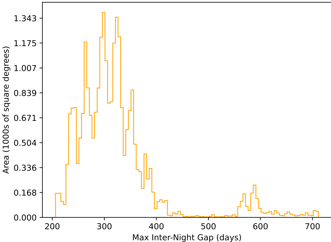
weather_cloudso30v3.4_10yrs All sky r band: Max Inter-Night Gap
