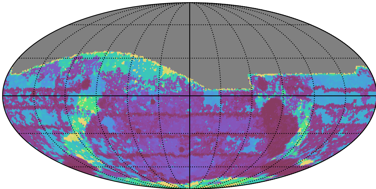
weather_cloudso30v3.4_10yrs All sky g band: Max Inter-Night Gap
