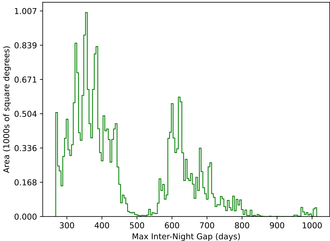
weather_cloudso30v3.4_10yrs All sky g band: Max Inter-Night Gap
