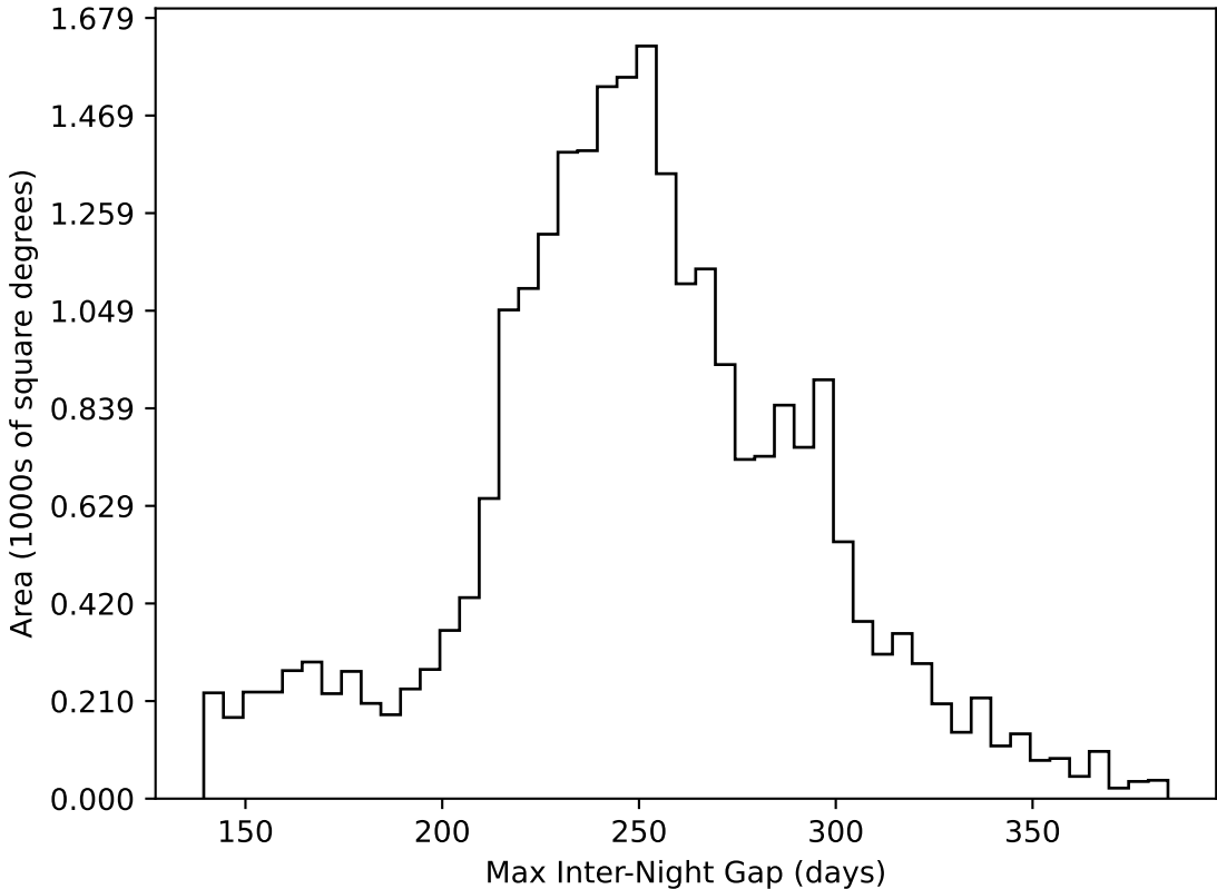
weather_cloudso30v3.4_10yrs All sky all bands: Max Inter-Night Gap
