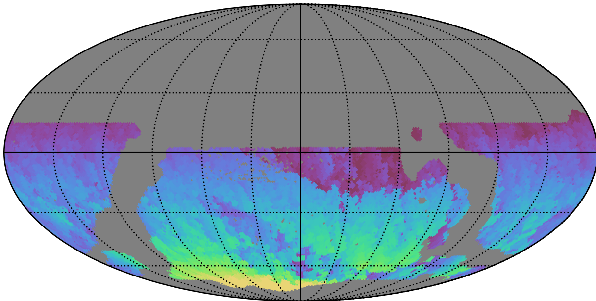
weather_cloudso30v3.4_10yrs WFD z band: Max HA
