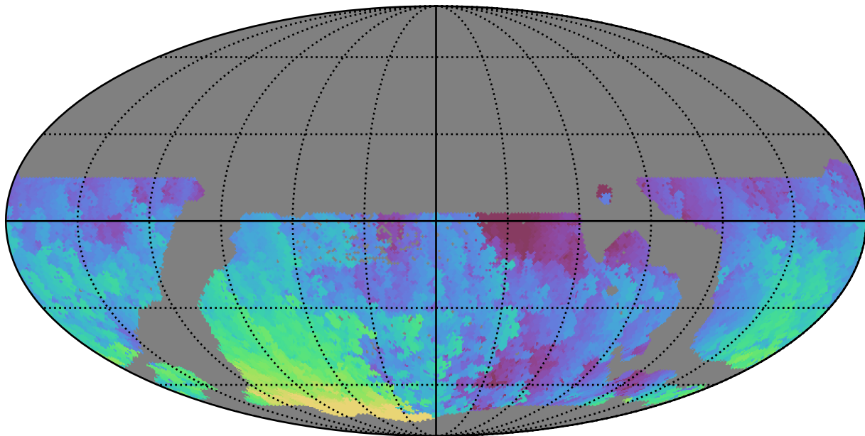
weather_cloudso30v3.4_10yrs WFD u band: Max HA
