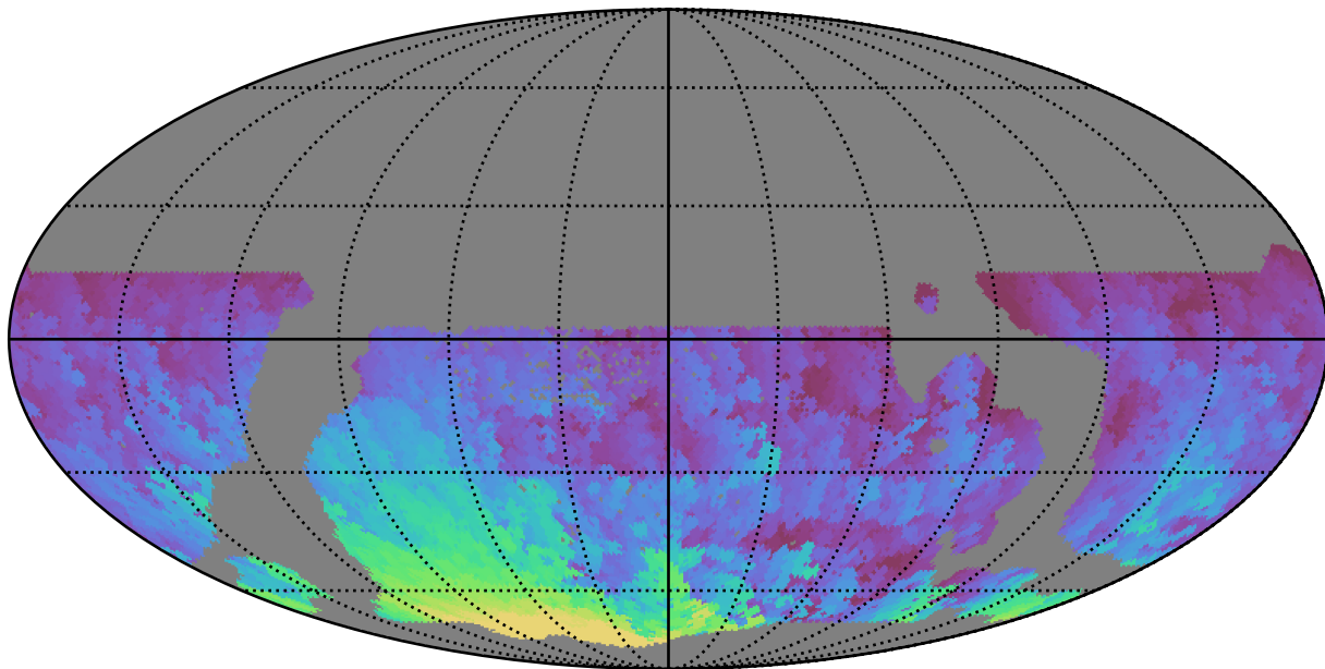
weather_cloudso30v3.4_10yrs WFD r band: Max HA
