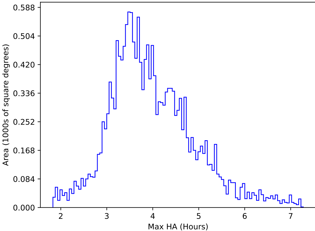
weather_cloudso30v3.4_10yrs WFD g band: Max HA
