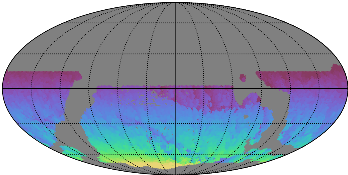
weather_cloudso30v3.4_10yrs WFD all bands: Max HA
