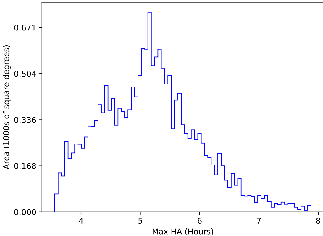
weather_cloudso30v3.4_10yrs WFD all bands: Max HA
