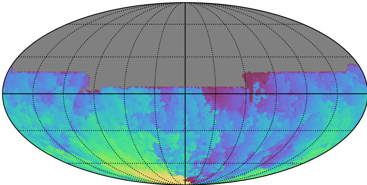
weather_cloudso30v3.4_10yrs All sky u band: Max HA
