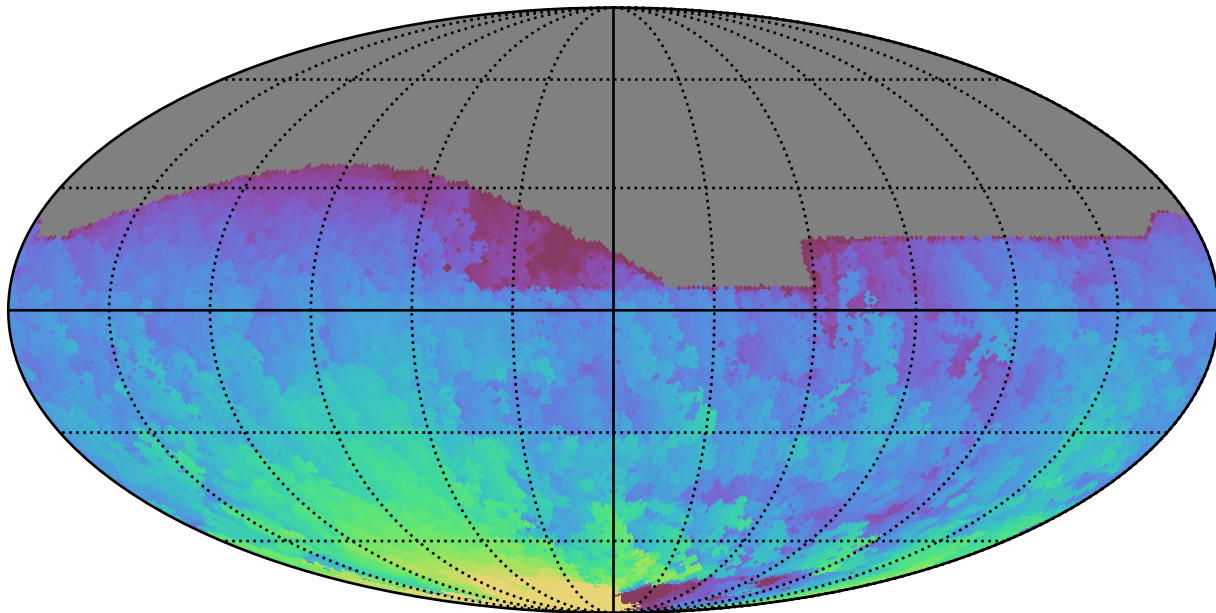
weather_cloudso30v3.4_10yrs All sky r band: Max HA
