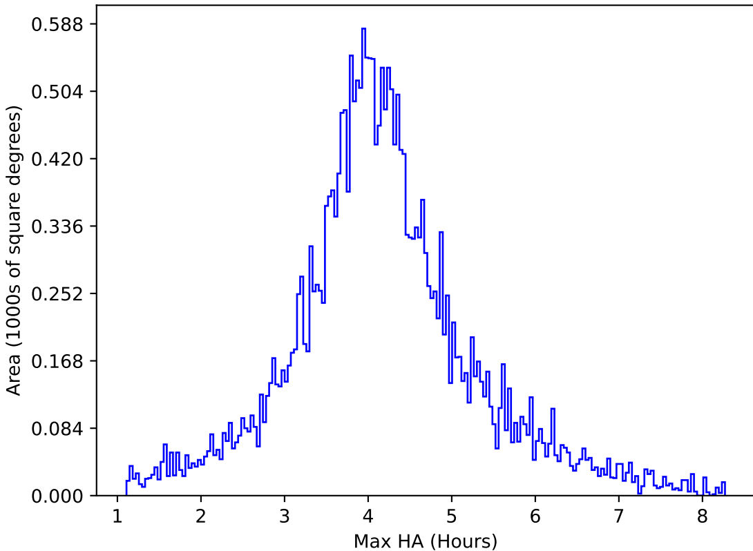
weather_cloudso30v3.4_10yrs All sky r band: Max HA
