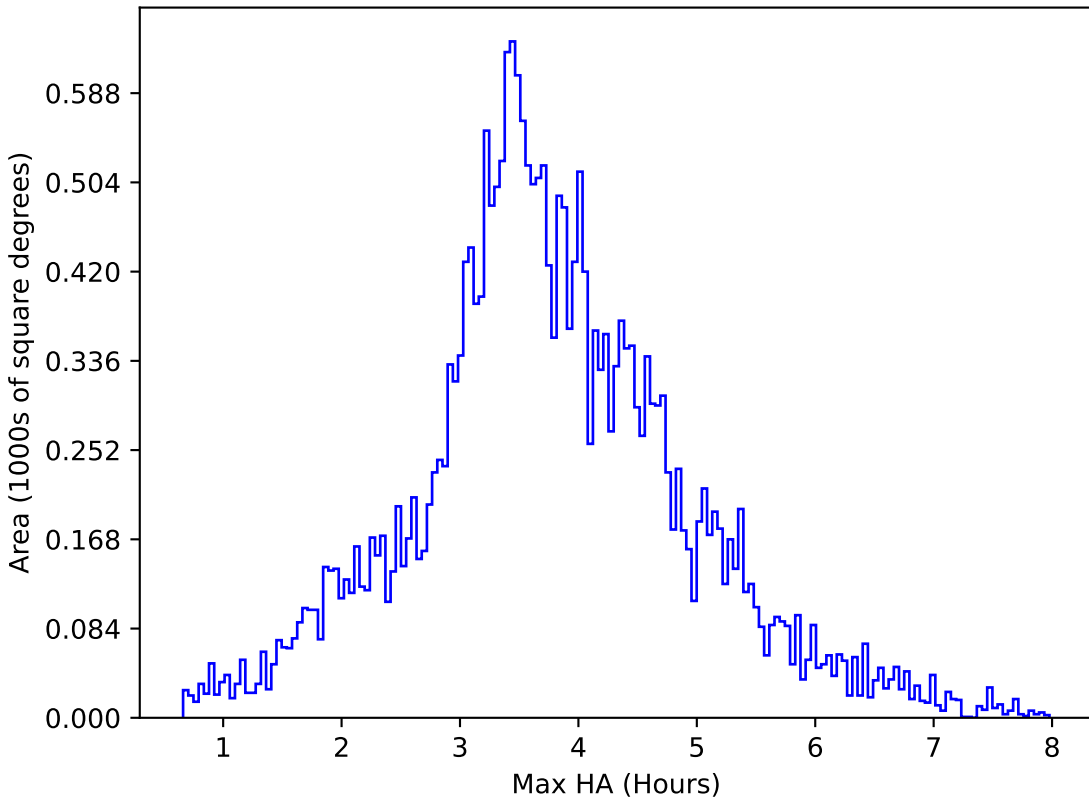
weather_cloudso30v3.4_10yrs All sky g band: Max HA
