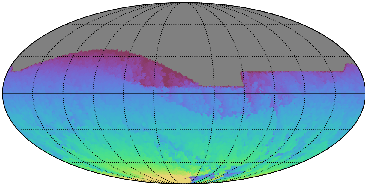
weather_cloudso30v3.4_10yrs All sky all bands: Max HA
