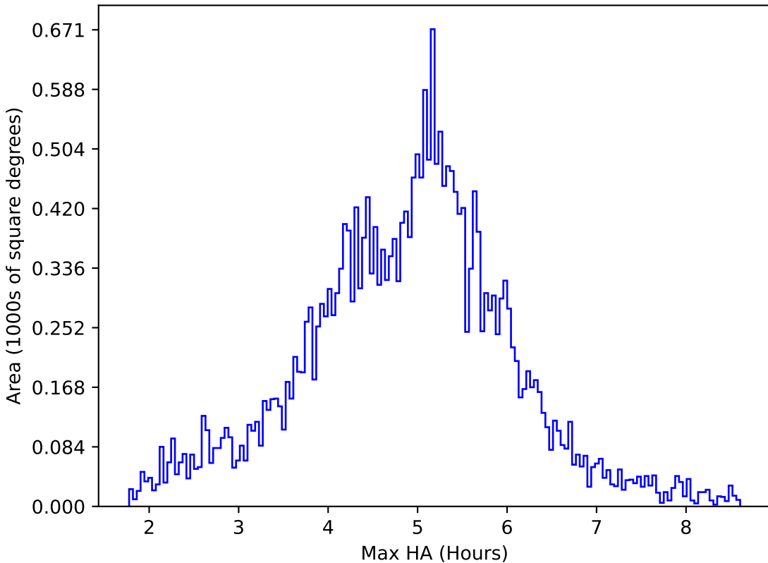
weather_cloudso30v3.4_10yrs All sky all bands: Max HA
