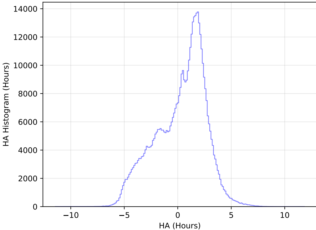
weather_cloudso30v3.4_10yrs WFD r band: HA Histogram
