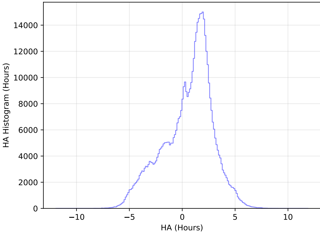
weather_cloudso30v3.4_10yrs WFD i band: HA Histogram
