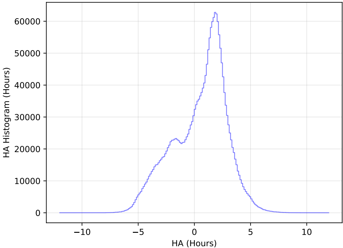
weather_cloudso30v3.4_10yrs WFD all bands: HA Histogram
