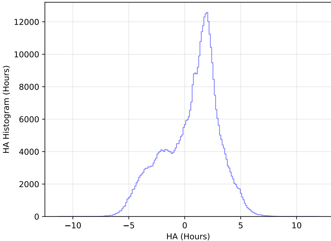
weather_cloudso30v3.4_10yrs All sky z band: HA Histogram
