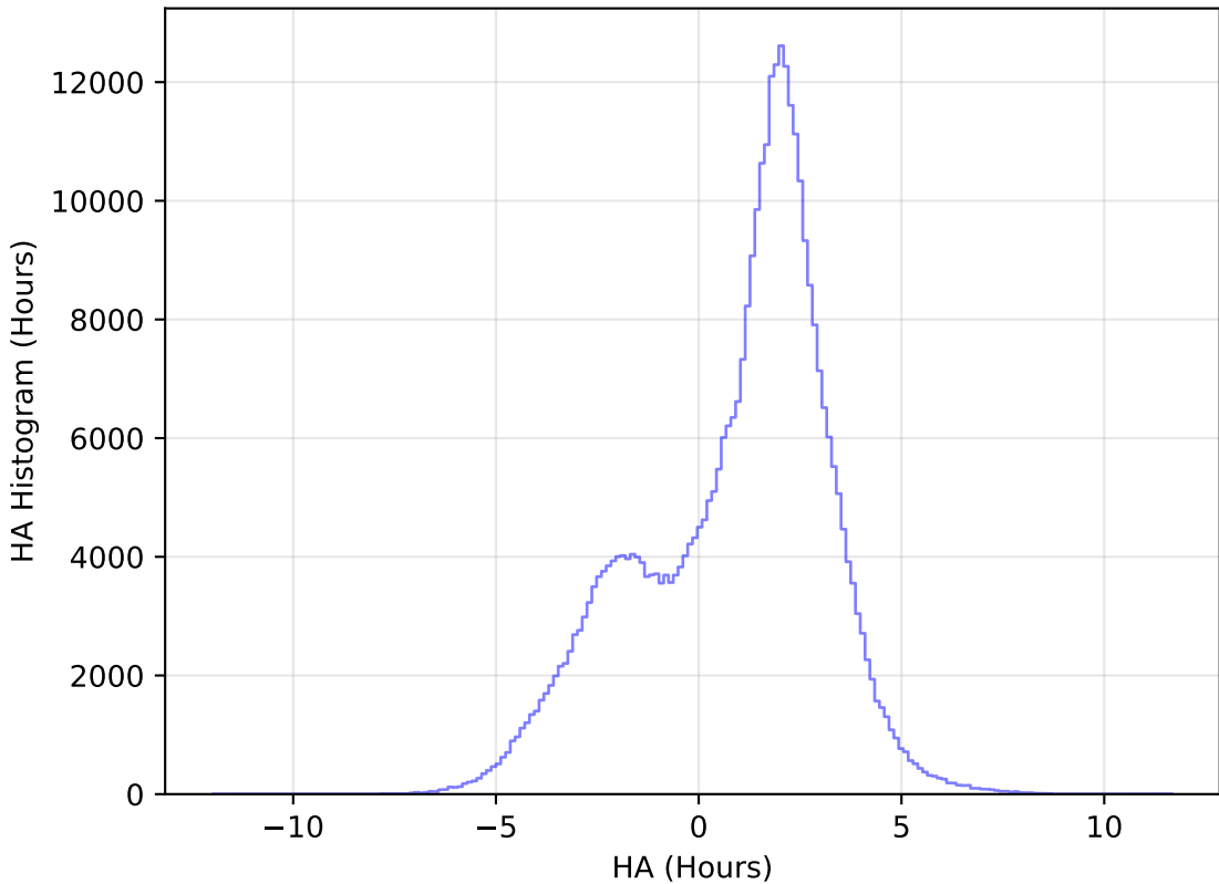
weather_cloudso30v3.4_10yrs All sky y band: HA Histogram
