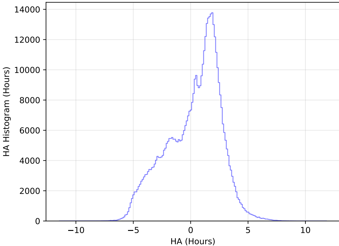
weather_cloudso30v3.4_10yrs All sky r band: HA Histogram
