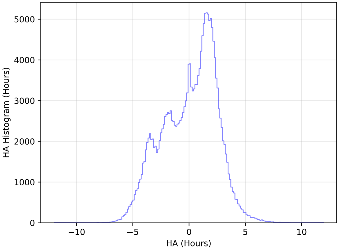
weather_cloudso30v3.4_10yrs All sky g band: HA Histogram
