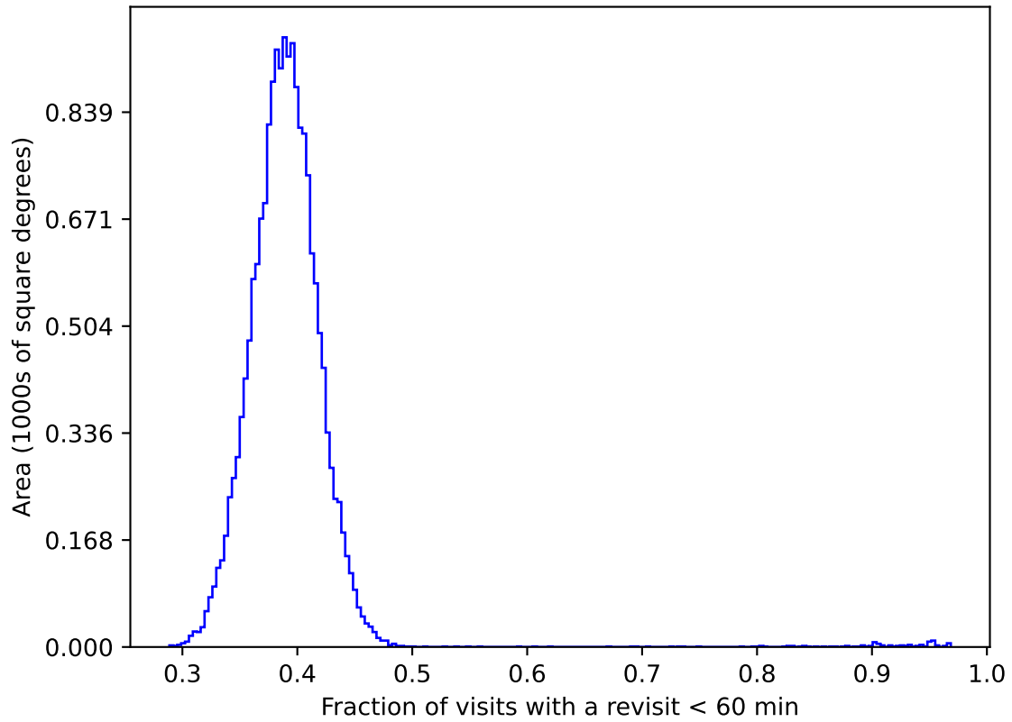
weather_cloudso30v3.4_10yrs gri WFD: Fraction of visits with a revisit < 60 min
