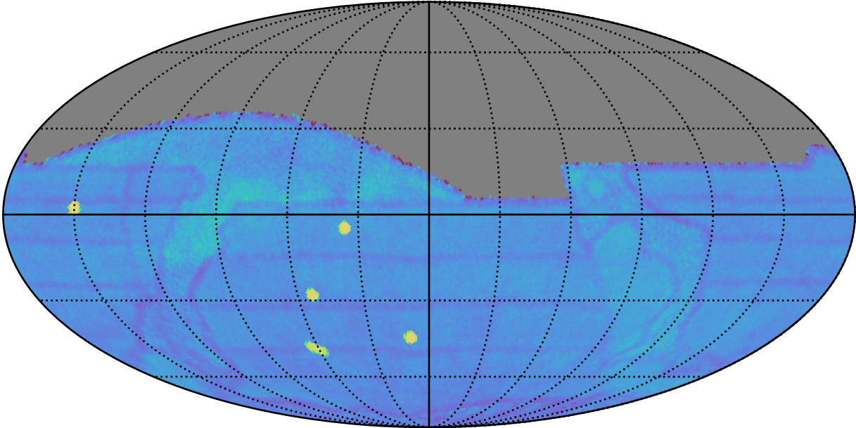
weather_cloudso30v3.4_10yrs gri All sky: Fraction of visits with a revisit < 60 min
