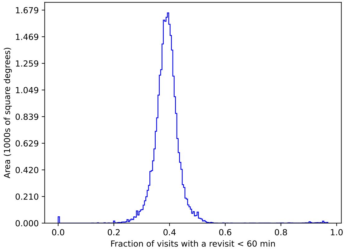
weather_cloudso30v3.4_10yrs gri All sky: Fraction of visits with a revisit < 60 min
