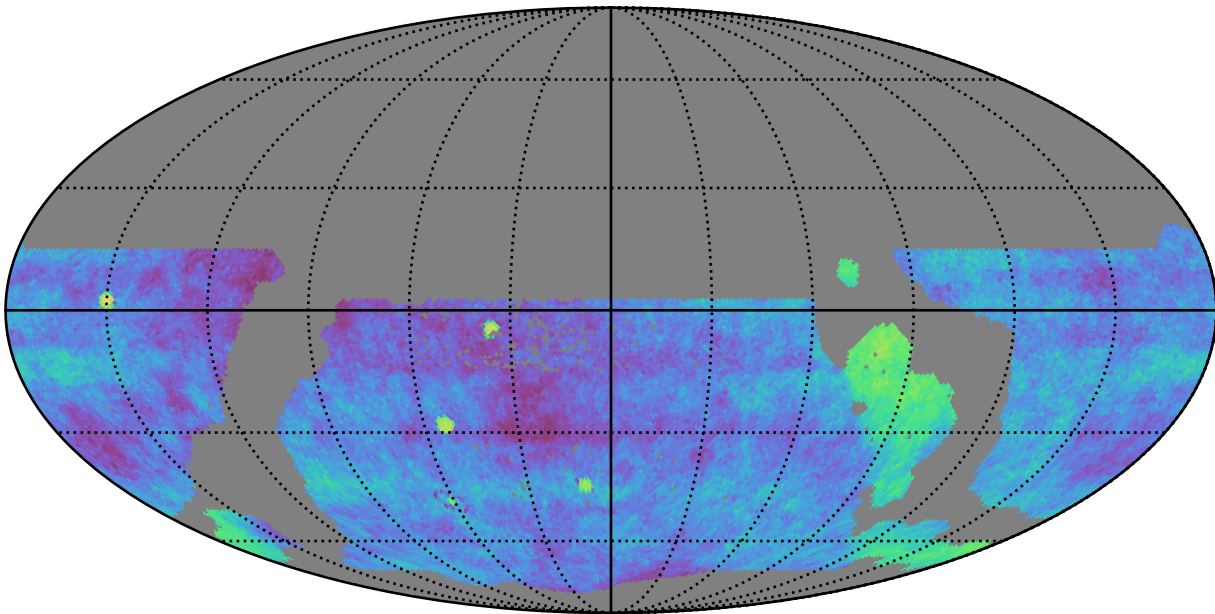
weather_cloudso30v3.4_10yrs gri WFD: Fraction of visits in pairs (20-90 min)
