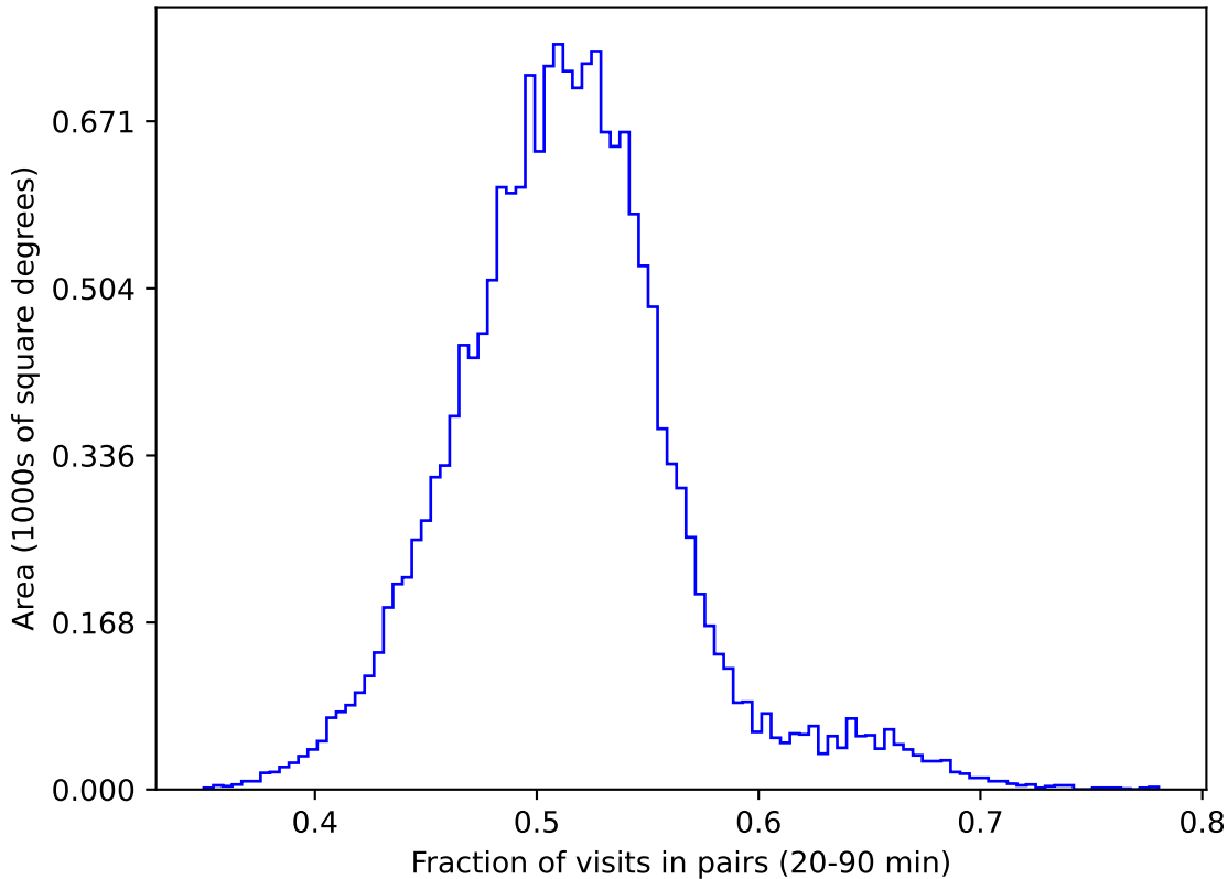
weather_cloudso30v3.4_10yrs gri WFD: Fraction of visits in pairs (20-90 min)
