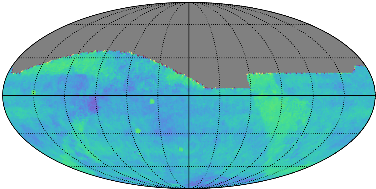
weather_cloudso30v3.4_10yrs gri All sky: Fraction of visits in pairs (20-90 min)
