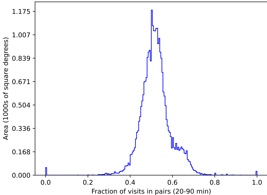
weather_cloudso30v3.4_10yrs gri All sky: Fraction of visits in pairs (20-90 min)
