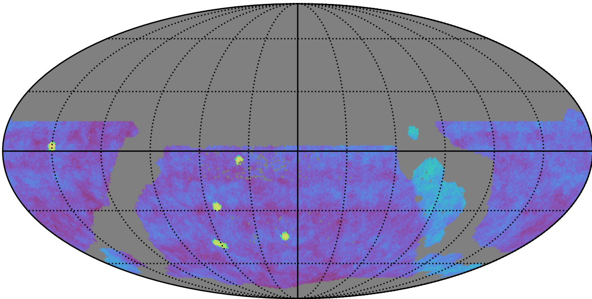
weather_cloudso30v3.4_10yrs gri WFD: Fraction of visits in pairs (10-60 min)
