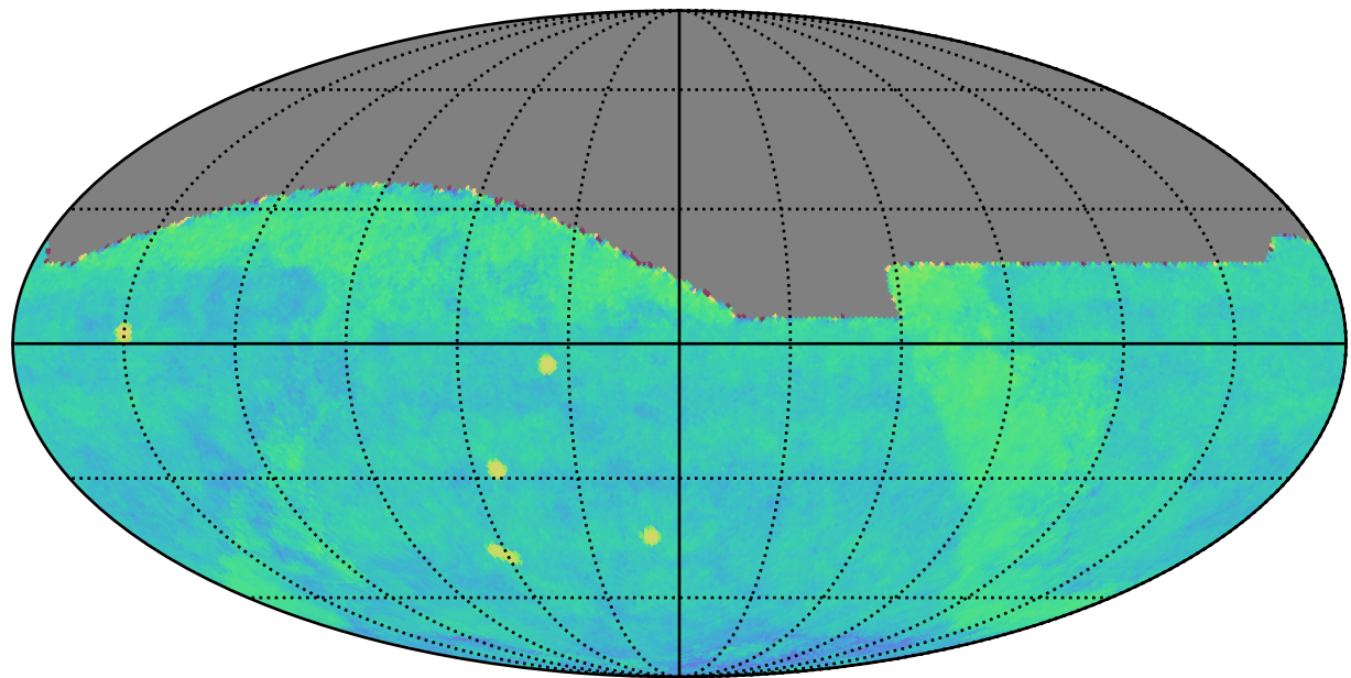
weather_cloudso30v3.4_10yrs gri All sky: Fraction of visits in pairs (10-60 min)
