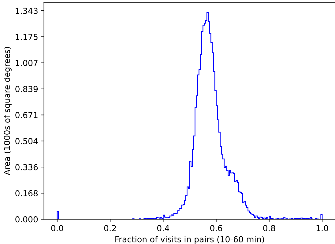
weather_cloudso30v3.4_10yrs gri All sky: Fraction of visits in pairs (10-60 min)
