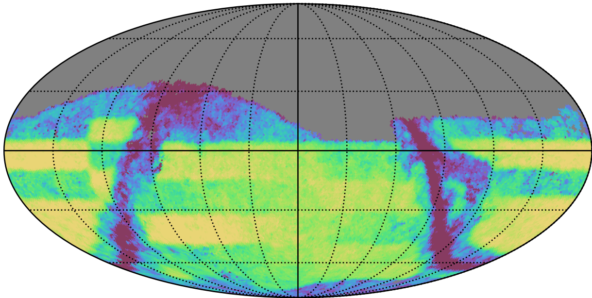
weather_cloudso30v3.4_10yrs Yr 3-4 z band: Exgal_CoaddM5
