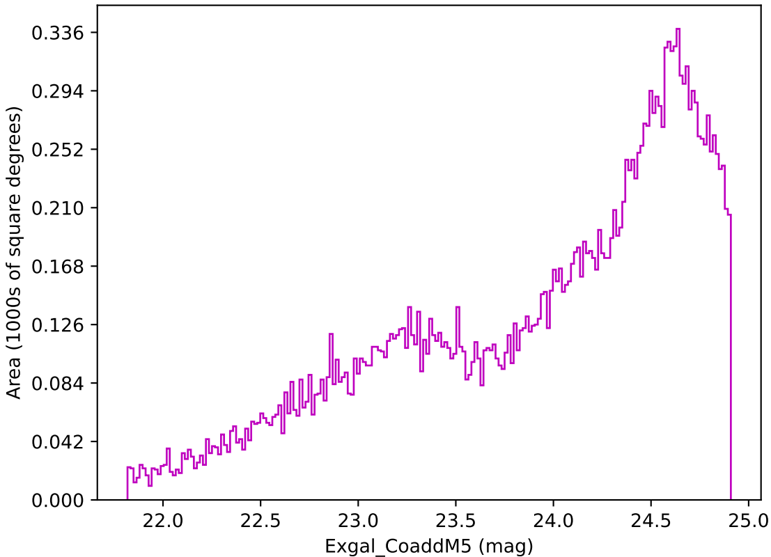
weather_cloudso30v3.4_10yrs Yr 3-4 z band: Exgal_CoaddM5
