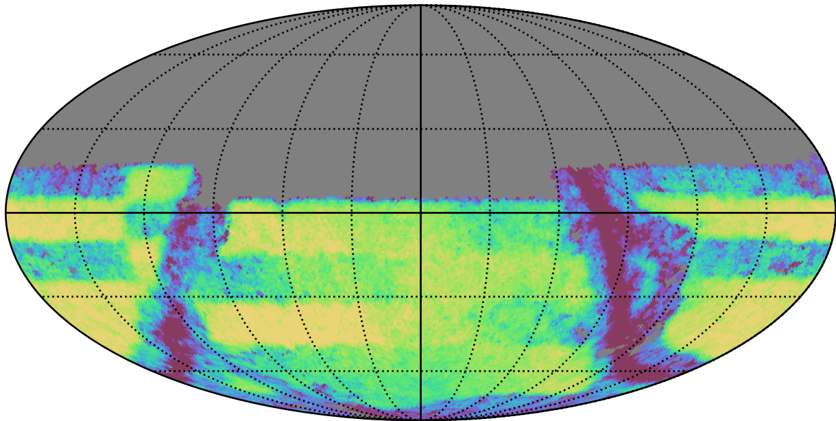
weather_cloudso30v3.4_10yrs Yr 3-4 y band: Exgal_CoaddM5
