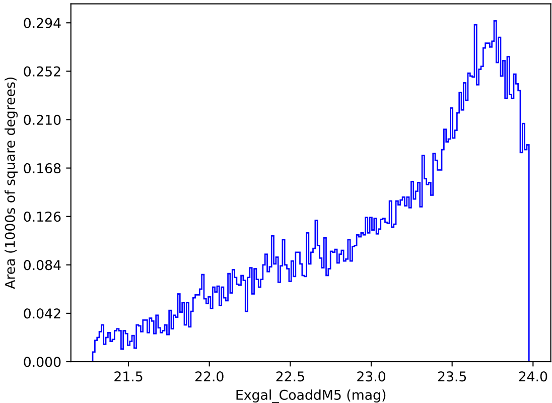
weather_cloudso30v3.4_10yrs Yr 3-4 y band: Exgal_CoaddM5
