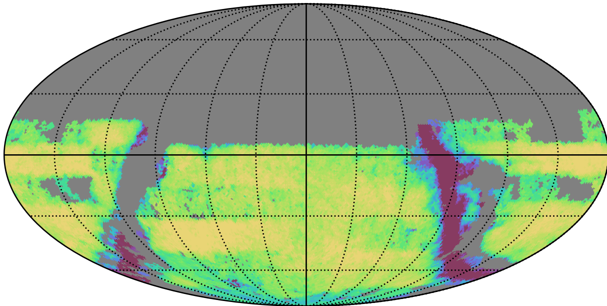
weather_cloudso30v3.4_10yrs Yr 3-4 u band: Exgal_CoaddM5
