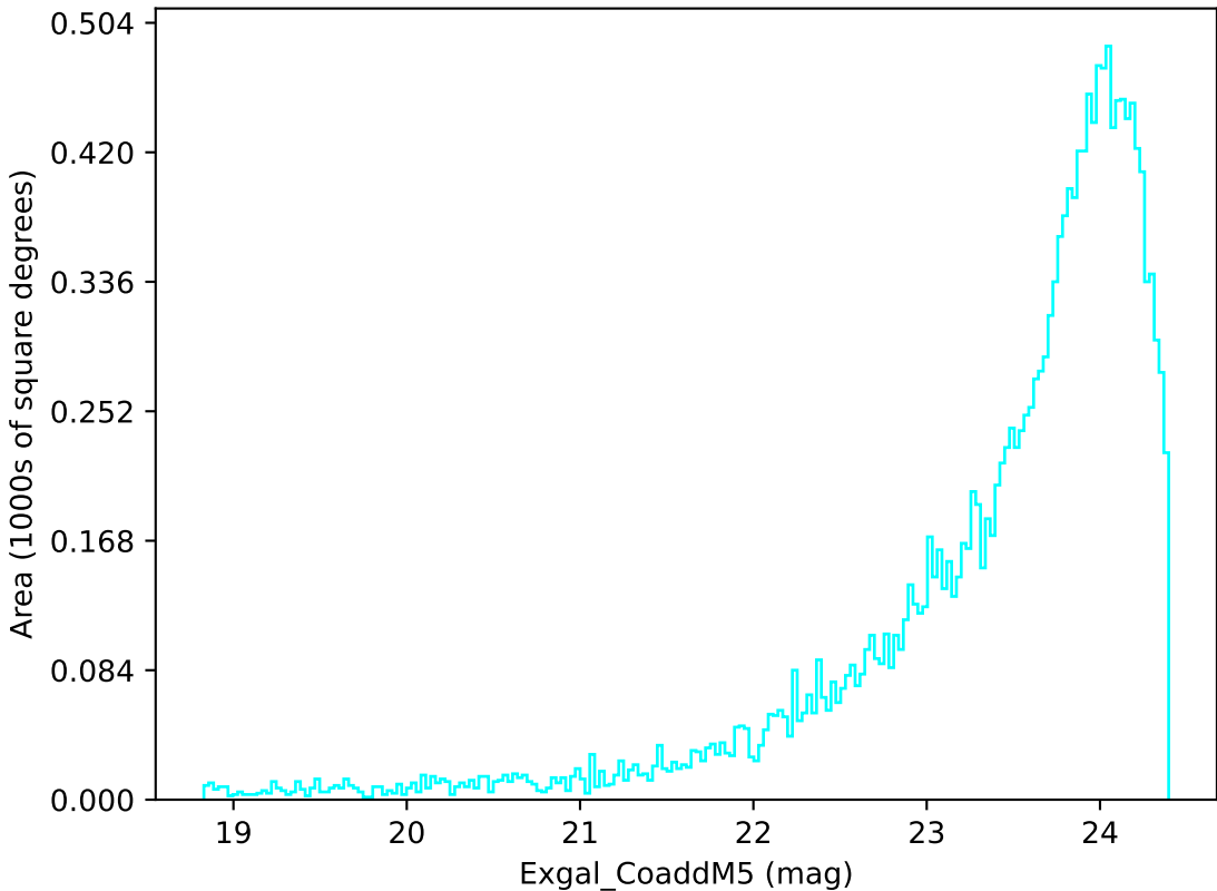
weather_cloudso30v3.4_10yrs Yr 3-4 u band: Exgal_CoaddM5
