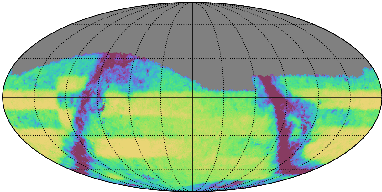
weather_cloudso30v3.4_10yrs Yr 3-4 r band: Exgal_CoaddM5
