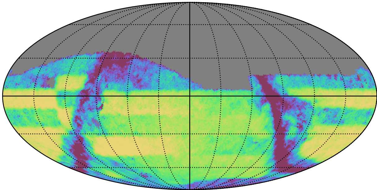
weather_cloudso30v3.4_10yrs Yr 3-4 i band: Exgal_CoaddM5
