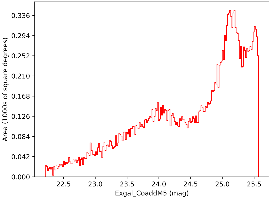
weather_cloudso30v3.4_10yrs Yr 3-4 i band: Exgal_CoaddM5
