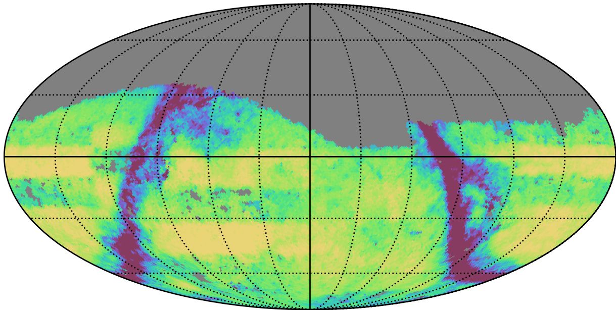
weather_cloudso30v3.4_10yrs Yr 3-4 g band: Exgal_CoaddM5
