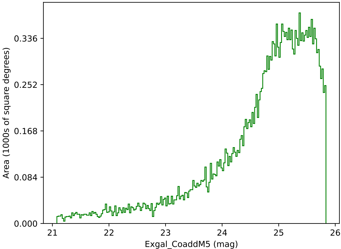
weather_cloudso30v3.4_10yrs Yr 3-4 g band: Exgal_CoaddM5
