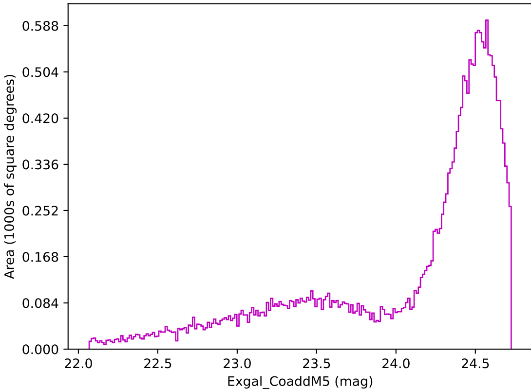
weather_cloudso30v3.4_10yrs Yr 1 z band: Exgal_CoaddM5
