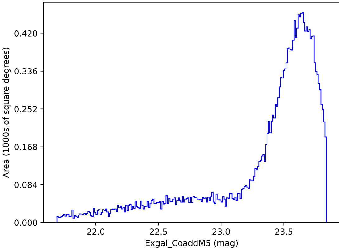
weather_cloudso30v3.4_10yrs Yr 1 y band: Exgal_CoaddM5
