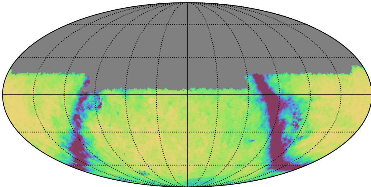
weather_cloudso30v3.4_10yrs Yr 1 u band: Exgal_CoaddM5
