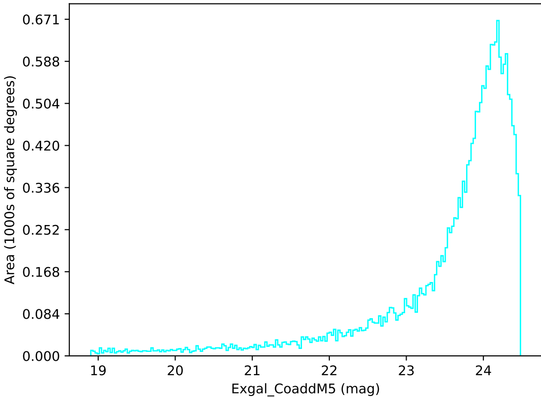
weather_cloudso30v3.4_10yrs Yr 1 u band: Exgal_CoaddM5
