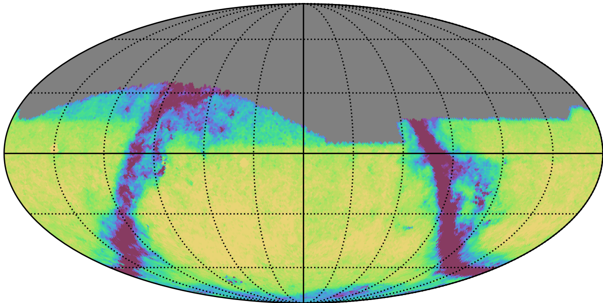
weather_cloudso30v3.4_10yrs Yr 1 r band: Exgal_CoaddM5
